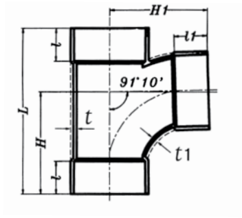
順T型同徑接頭 Sanitary Tee
