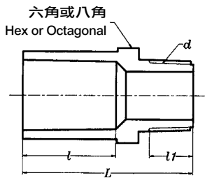
Male Adapter (Plastic Thread)
