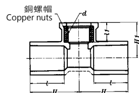
Faucet Fitting (Insert Bronze Nut) - Fixture Tee
