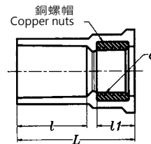
Faucet Fitting (Insert Bronze Nut) - Female Adapter
