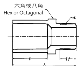
Male Adapter (Plastic Thread)
