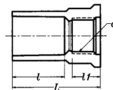
Faucet Fitting (Plastic Thread) - Female Adapter
